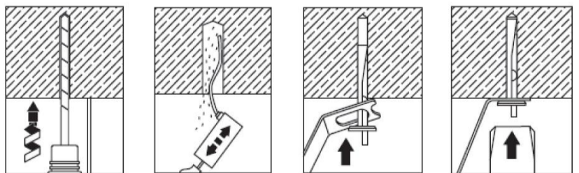
Drill hole with drill bit.
