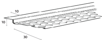
Typical wall Application
