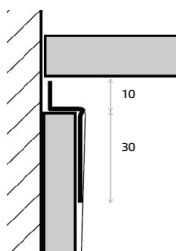
Typical wall Application
